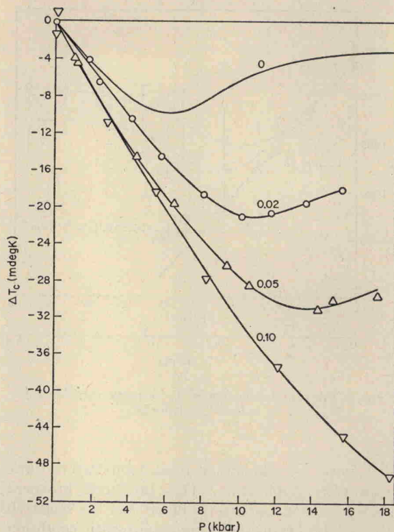
FIG. 6. \Delta T_c as a function of pressure for Re-W alloys. The number associated with each curve represents the at.% concentration of W.
