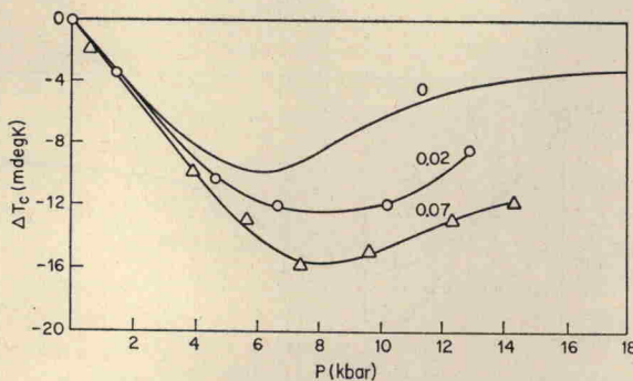
FIG. 7. \Delta T_c as a function of pressure for Re-Mo alloys. The number associated with each curve represents the at.% concentration of Mo.
